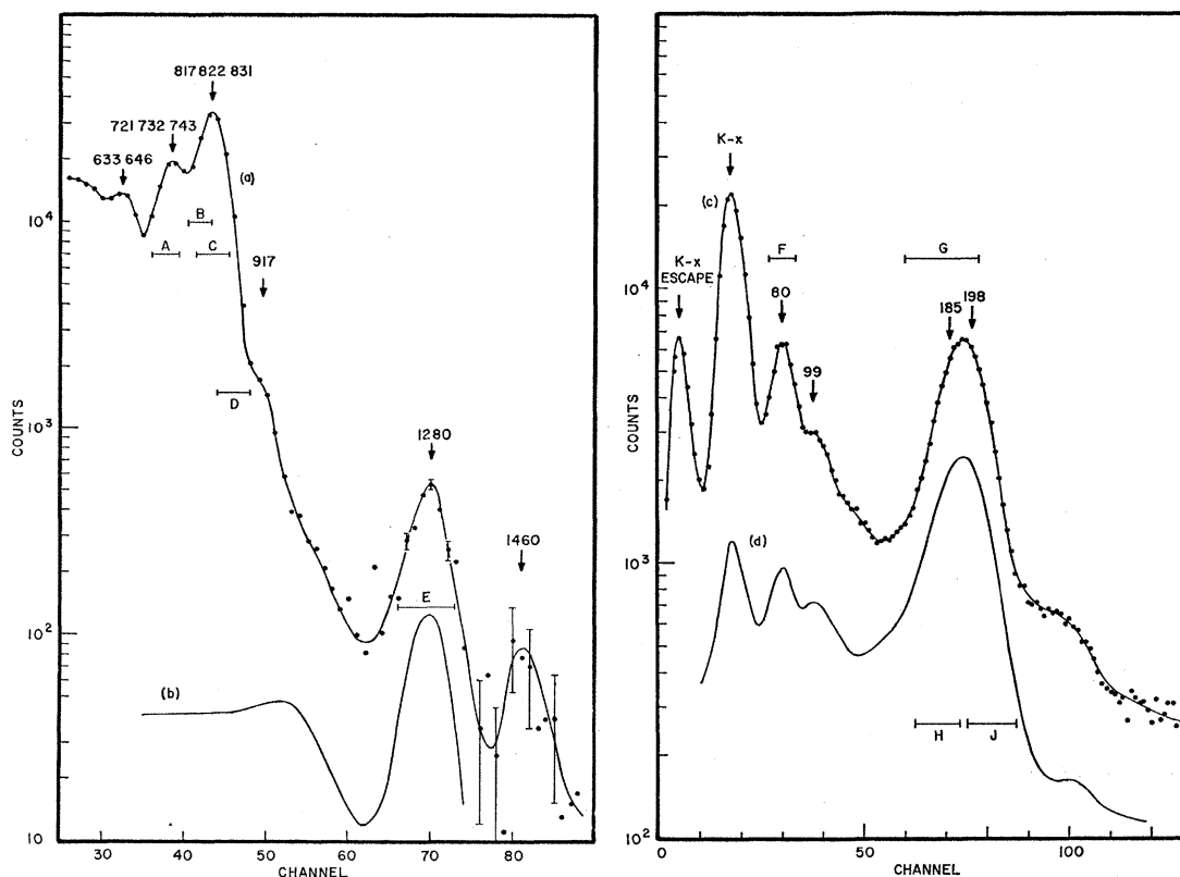
FIG. 6. Gamma-ray spectra and gates used for directional correlation measurements. Curve (a) shows a spectrum and gates (A-E) using a 2- \times 2-in. NaI crystal; (b) a 1280-keV contour ( \text{Na}^{22} ) for the same geometry as (a); (c) a spectrum and gates (F,G) using a 4-mm \times 1-in. NaI crystal; and (d) a spectrum and gates (H,J) using a 1- \times \frac{1}{2} -in. crystal.
