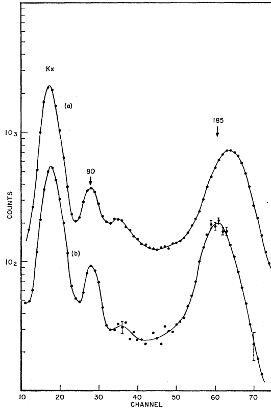
FIG. 5. Gamma-ray spectrum in coincidence with the 1280-keV gamma transition. Curve (a) shows the singles spectrum and curve (b) shows the coincidence spectrum (corrected for chances).
