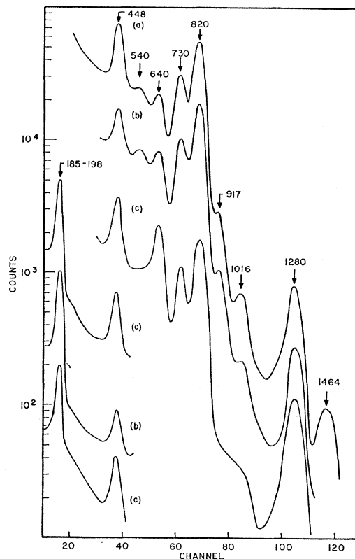
FIG. 2. Gamma-ray coincidence spectra obtained when gating electrons of ~80 keV (detected in a \frac{1}{8} -in.-thick Pilot B scintillator). Curve (a) shows a singles spectrum from 150–1500 keV, (b) the coincidence spectrum with a gate set on the 80- L internal conversion electron peak, and (c) the coincidence spectrum with the gate set on the region around 150 keV.
